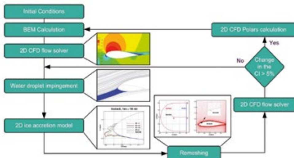
Figure 5 Simulation workflow for assessing rotor performance under icing conditions; Image: AIT
